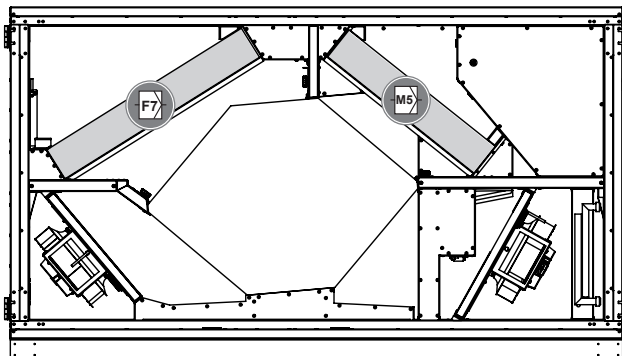
Abb. 24: Position Luftfilter
